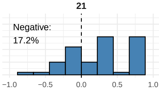
Spearman's rank correlation coefficient
